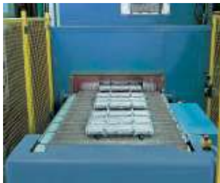
Installation de brasage CAB (Controlled Atmosphere Brazing)
